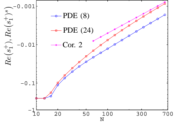
Fig. 4. The least stable eigenvalue of the governing PDE (8) and of the self-adjoint PDE (24) with k_m(x) = k_m^*(x) , and the predictions of Corollary 2 for the self-adjoint PDE for N > 50 . The parameters are k_0 = 1 , b_0 = 0.5 , and \epsilon \approx 0.35 . Consistent with Lemma 2, the least stable eigenvalue of the self-adjoint PDE upper bounds that of the original non self-adjoint problem. Moreover, Corollary 2 predicts the least stable eigenvalue of the self-adjoint PDE quite accurately for large N .
