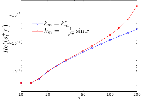
Fig. 3. Real part of the least stable eigenvalue of the self-adjoint PDE (24) with the optimal mistuning profile and sinusoidal profile. The parameters are k_0 = 1 , b_0 = 0.5 , and \epsilon \approx 0.35 . As predicted, the optimal mistuning profile results in a smaller eigenvalue compared to that from a sinusoidal one.
