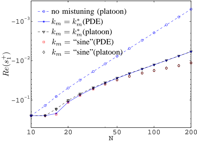
Fig. 5. Least stable eigenvalues of the mistuned PDE (8) as well as that of the discrete platoon with sinusoidal mistuning profile, and k_m^* mistuning profile (optimal for the self-adjoint problem (24)). The legend “(platoon)” means that the eigenvalues are those of the state matrix for (1)-(2), whereas “(PDE)” means that the eigenvalues are of the governing PDE (4). Also shown are the least stable eigenvalues of the closed loop platoon without any mistuning (i.e., symmetric bidirectional control). “sine” denotes k_m(x) = -\frac{1}{\sqrt{\pi}} \sin(x) . The parameters are k_0 = 1 , b_0 = 0.5 , and \epsilon = 0.35 , which results in the mistuned gains differing from the nominal (symmetric bidirectional) case by \pm 10\% . The eigenvalues of the discrete platoon match the eigenvalues of the discrete platoon accurately, but the optimal profile designed for the self-adjoint problem does not perform as well for the original non self-adjoint problem as the sinusoidal profile.
