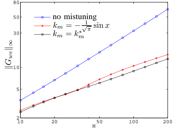
Fig. 6. H_\infty norm of the transfer function G_{we} from disturbance w to spacing error e for three cases: without mistuning, with sinusoidal mistuning, and with k_m^* mistuning. The H_\infty norms are significantly lower with mistuning than with none (i.e., symmetric bidirectional control), even though the mistuning was only \pm 10\% ( \epsilon = 0.35 ).
